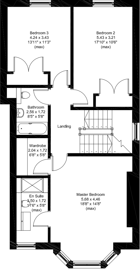
UNIT 6 : FIRST FLOOR
