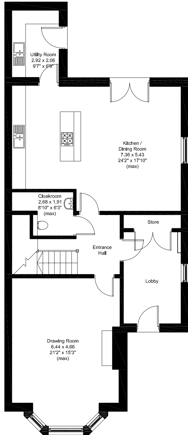
UNIT 4 : GROUND FLOOR
