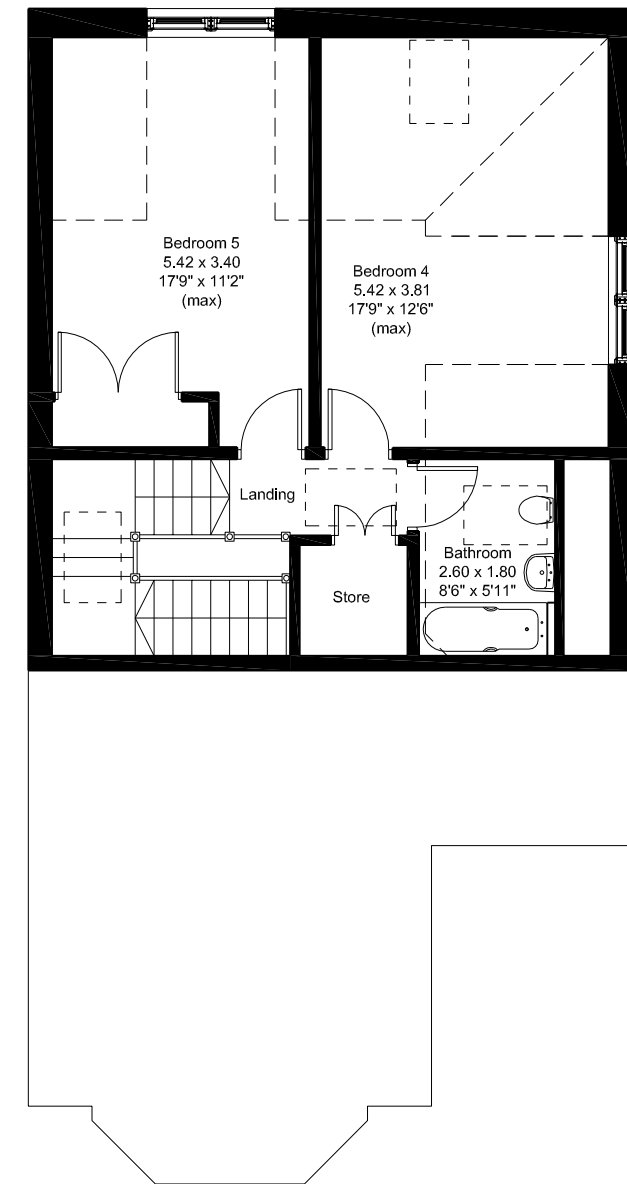
UNIT 4 : SECOND FLOOR
