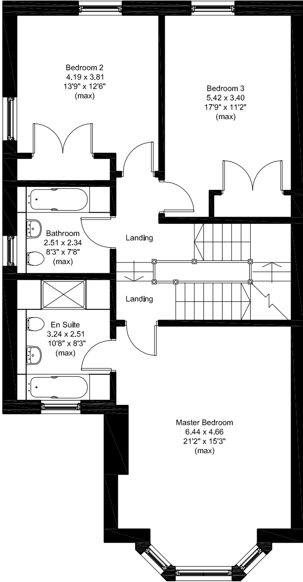
UNIT 12 : FIRST FLOOR
